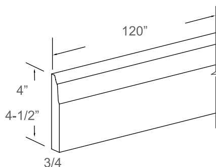
BASE MOLDING
